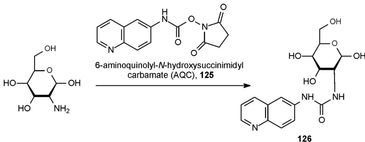
Scheme 24. Scheme for the preparation of AQC derivatives.
