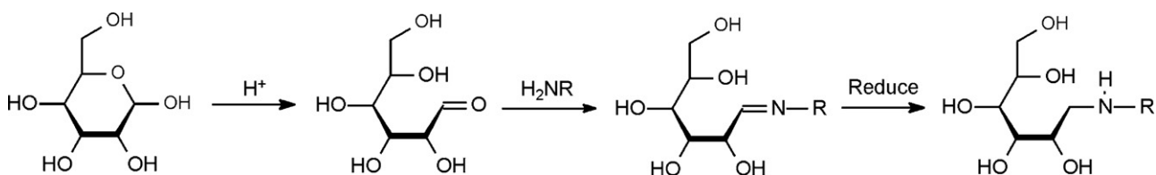
Scheme 5. Amines used to form Schiff bases of carbohydrates.
