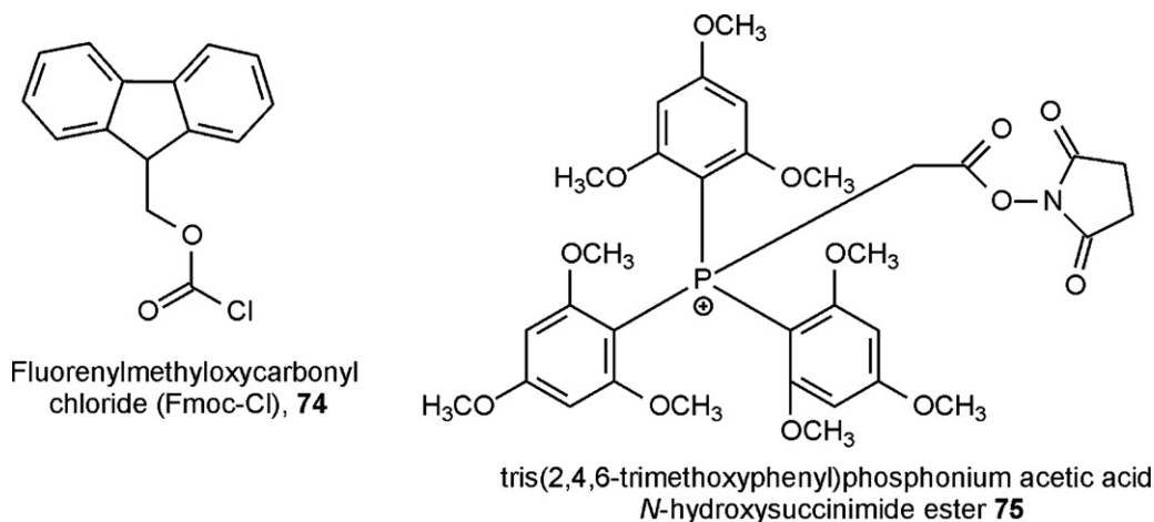
Scheme 12. Structure of fluorenylmethoxycarbonyl chloride (Fmoc-Cl) and the TMPP reagent.
